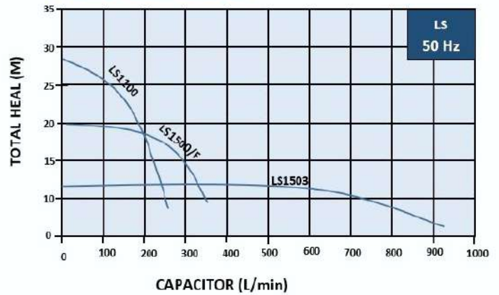
Performance Curve:
